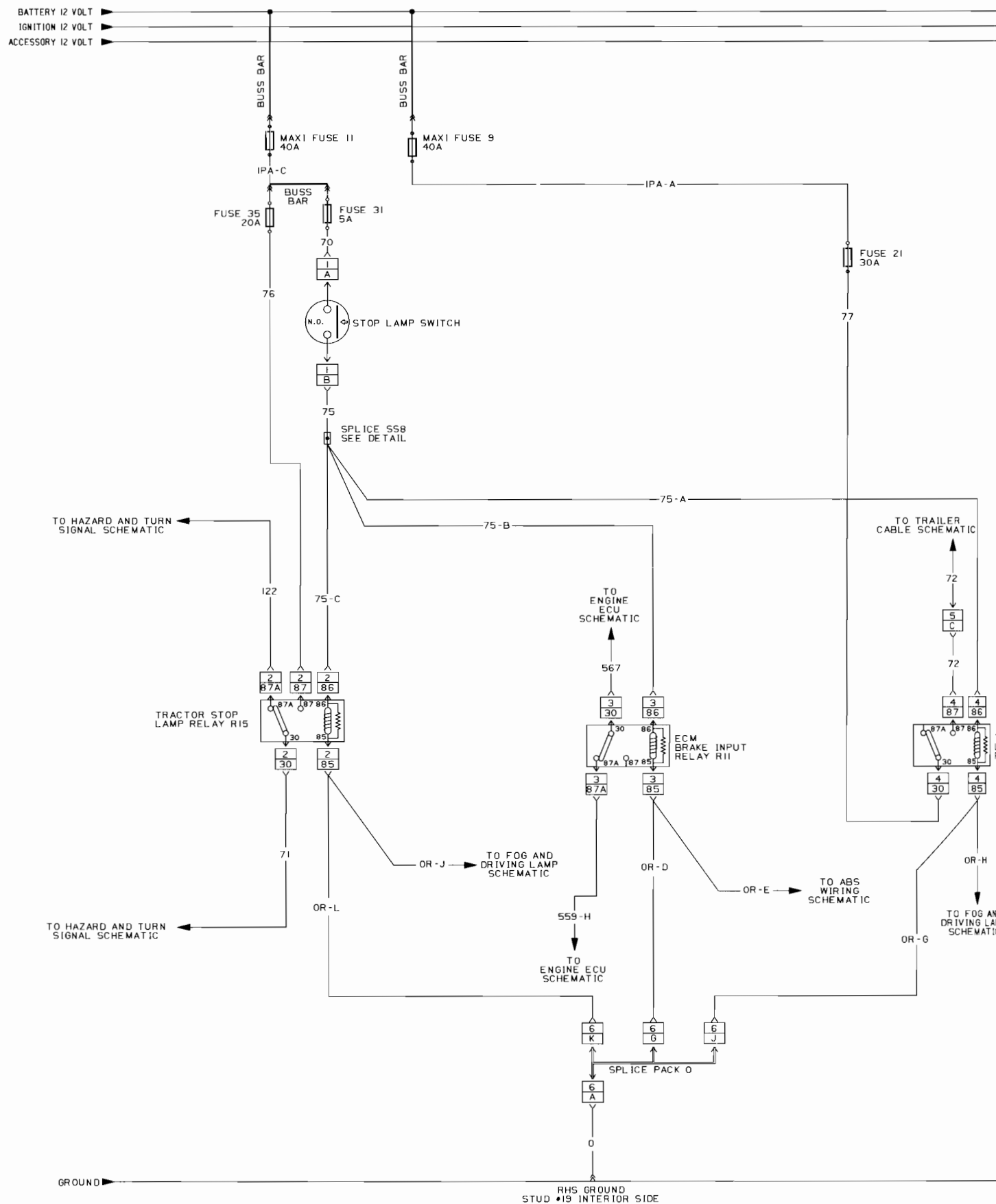
Stop Lamps, Caterpillar 3406E, Cummins M11/N14 Plus and Detroit Diesel Series
