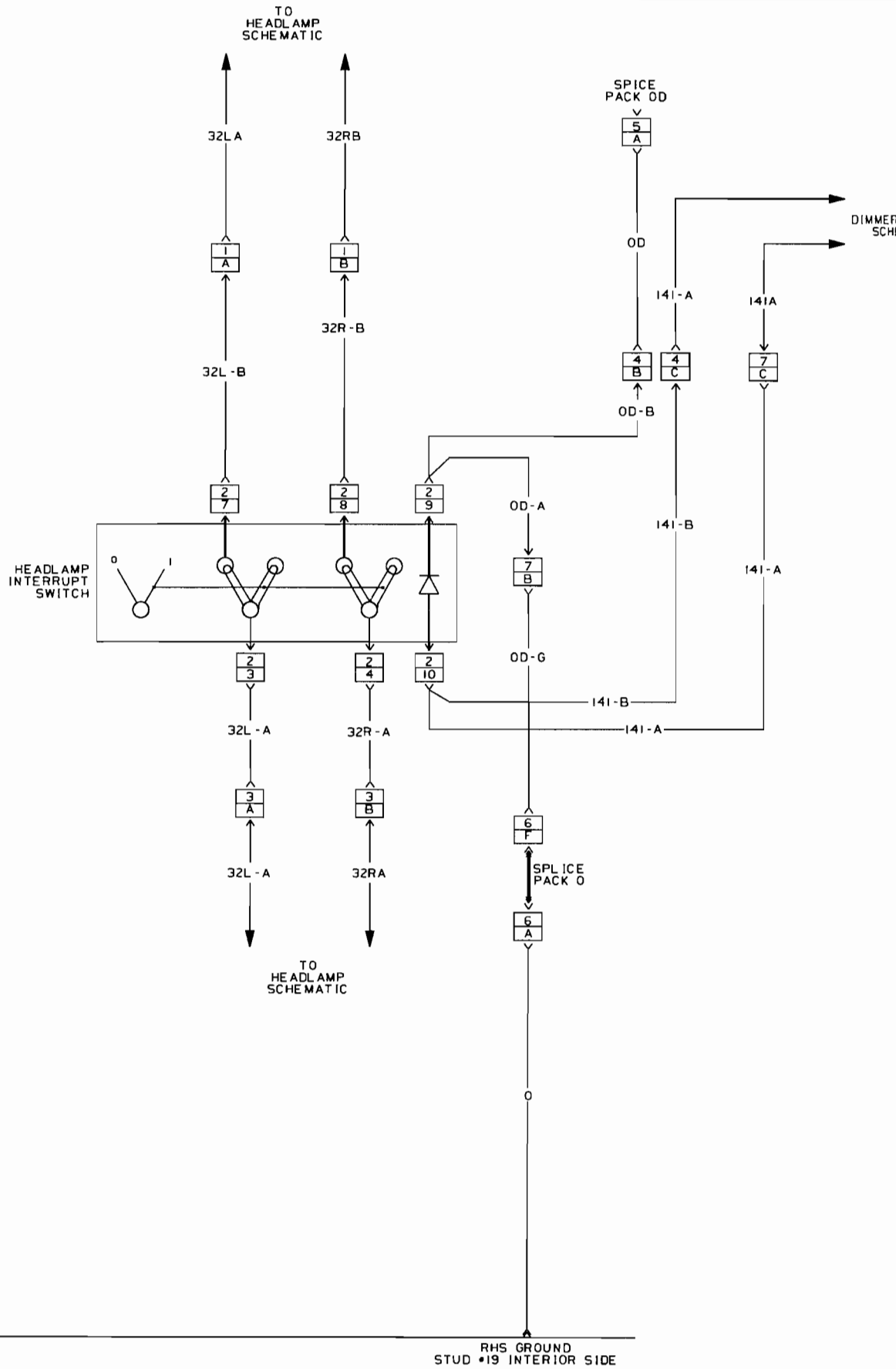
Headlamp Interrupt Switch - VNL, VNM
